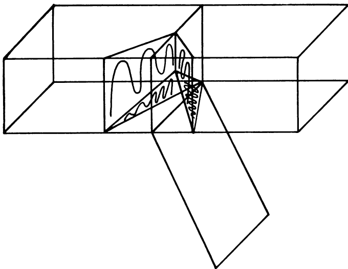
FIGURE 5. After unfolding flanges (\psi_\varepsilon^{-1}) . Final image of Z_2 (h_\varepsilon \circ \bar{g}_\varepsilon(Z_2)) , indicating images of A and F_1 .
