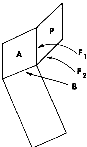
FIGURE 3. Image after straightening A ( \alpha_e ) and "folding flanges" into central plate P ( \psi_e ). (Motion pointwise fixed on B , F_1 , and F_2 .)
