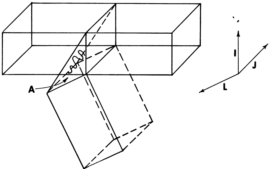
FIGURE 2. Image after "projecting" ( \tilde{g}_\epsilon ).
