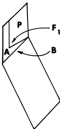
FIGURE 4. After absorbing A into P carrying B onto F_2 ( \beta_e ).
